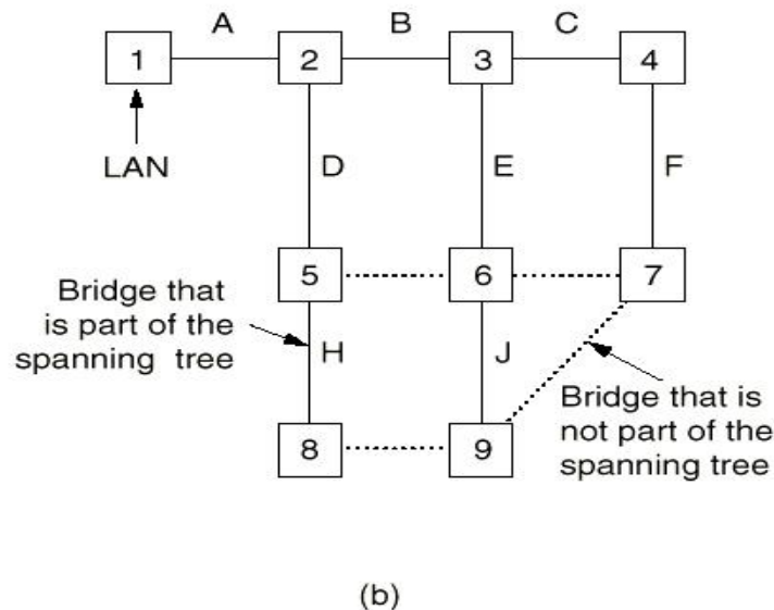
Fig. 4-40. (a) Interconnected LANs. (b) A spanning tree covering the LANs. The dotted lines are not part of the spanning tree.
