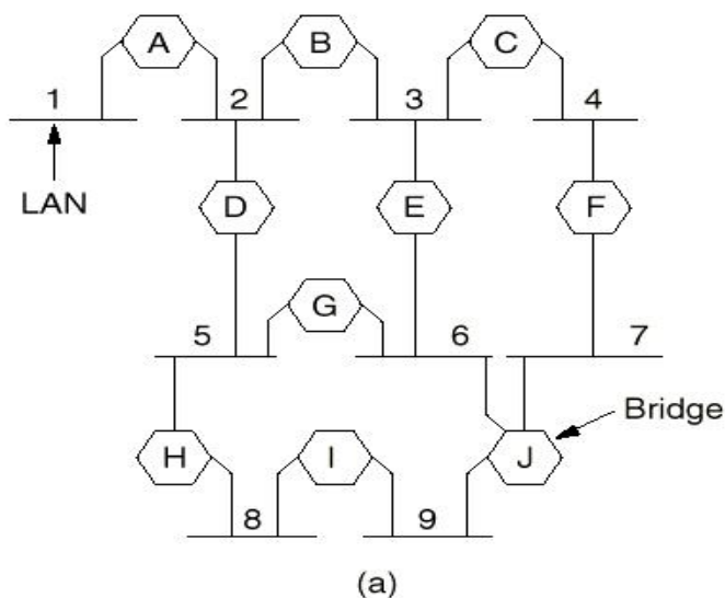
Fig. 4-40. (a) Interconnected LANs. (b) A spanning tree covering the LANs. The dotted lines are not part of the spanning tree.
